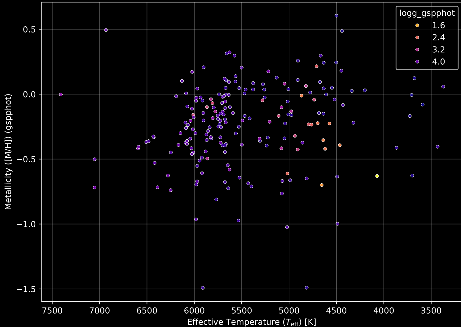
APOGEE DR17 Field: [080+66_MGA] Stellar Population Parameters (n= 201)
